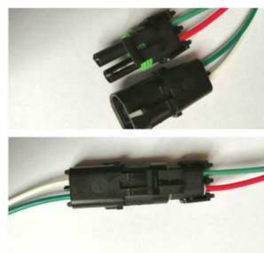
Kit Weather pack ensamblado 2 via CA44
