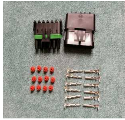
Kit aguja de 6 vias kit weather pack 6 pines CA127
